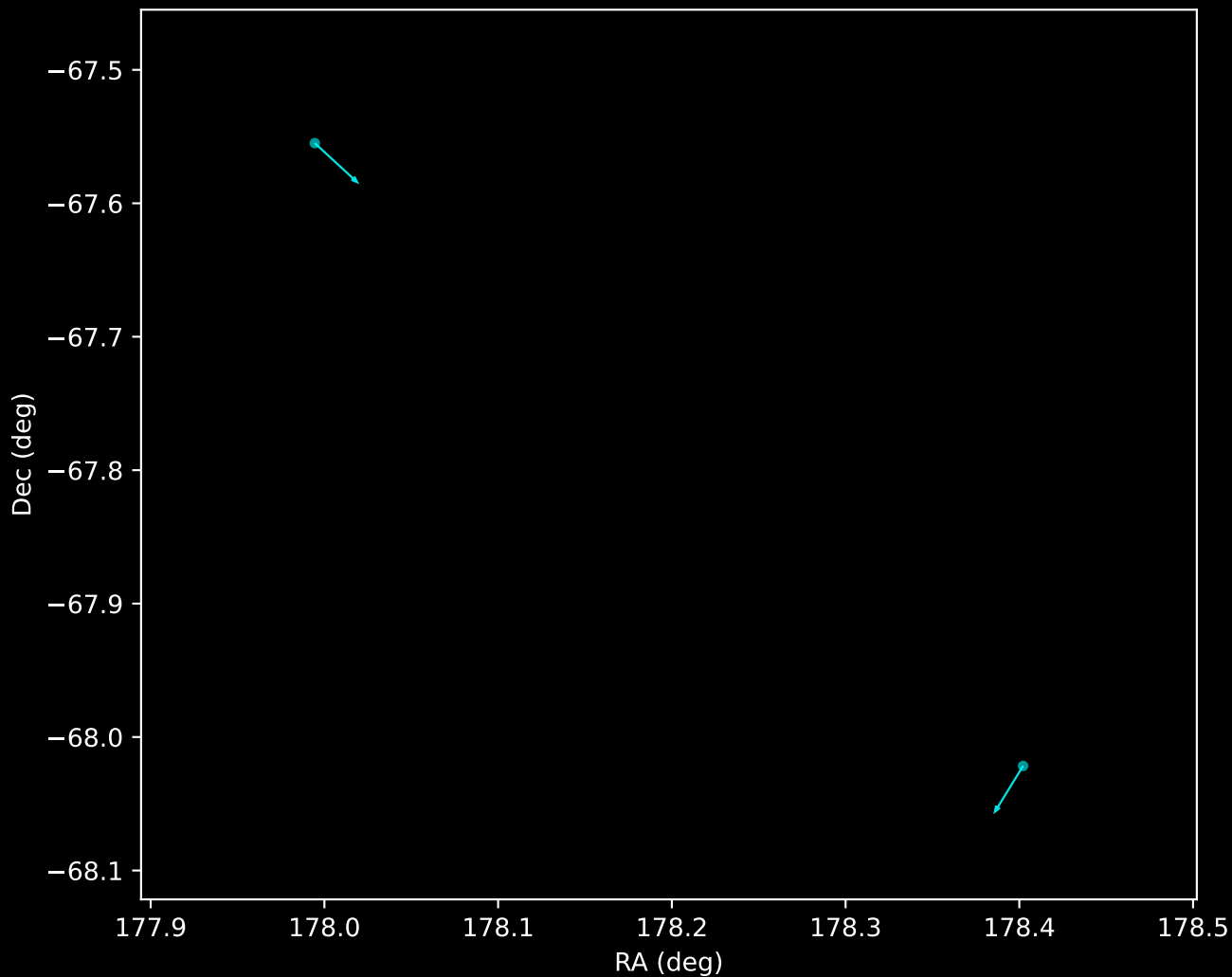
APOGEE DR17 Noise Stream Proper Motion Vectors (n=2)
