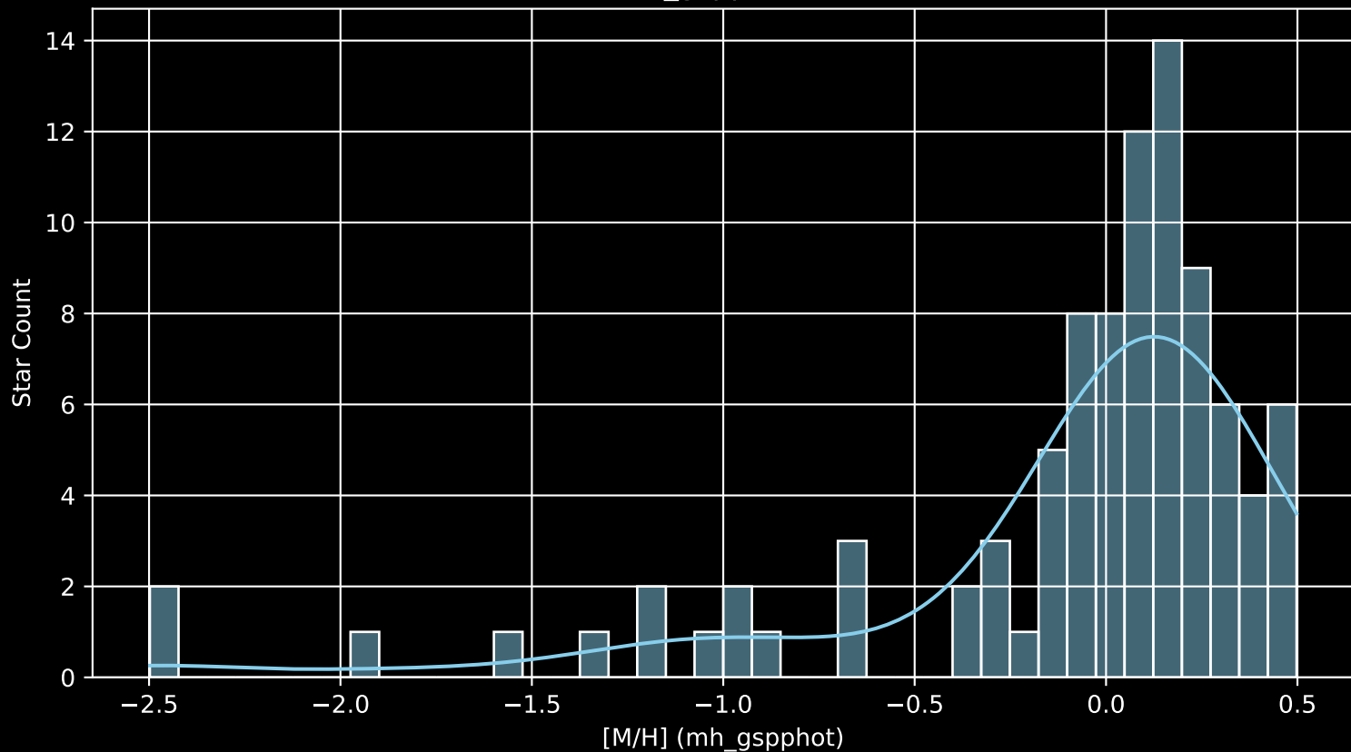
APOGEE DR17 Field: [LMC27 [M/H] (mh_gspphot) (n= 92)
