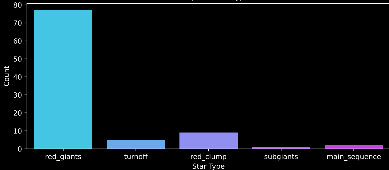
APOGEE DR17 Field: [LMC27] Count plot of Star Type
