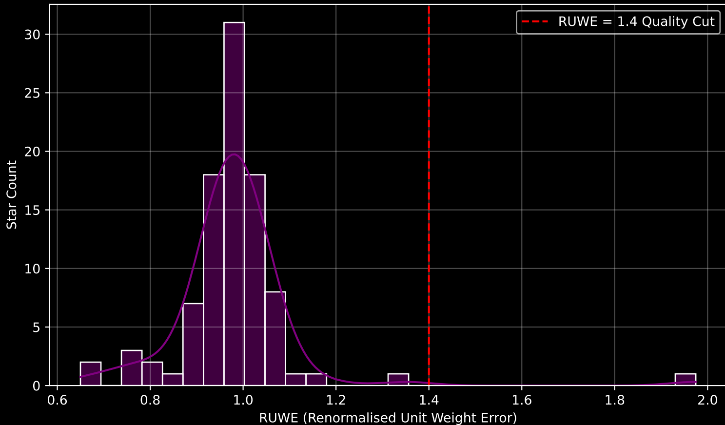
GAPOGEE DR17 Field [LMC27] RUWE Distribution (n= 94)
