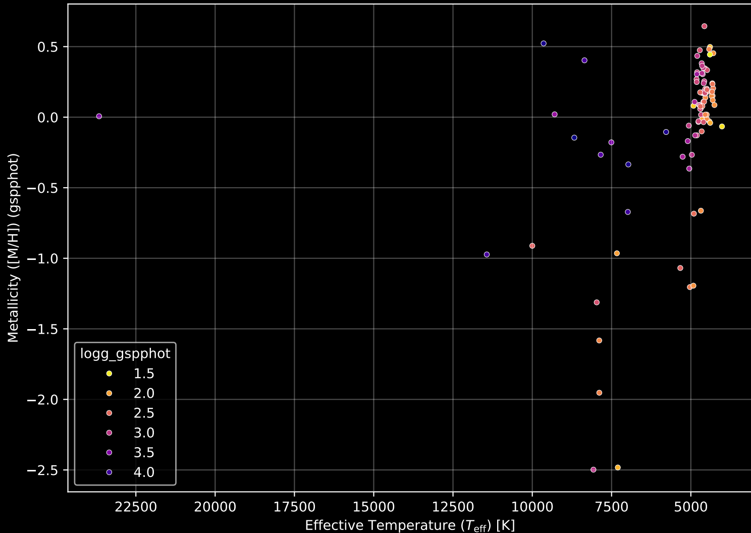
APOGEE DR17 Field: [LMC27] Stellar Population Parameters (n= 94)
