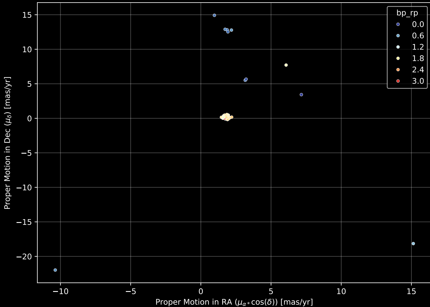
APOGEE DR17 Field: [LMC27] Proper Motion Diagram (n= 94)
