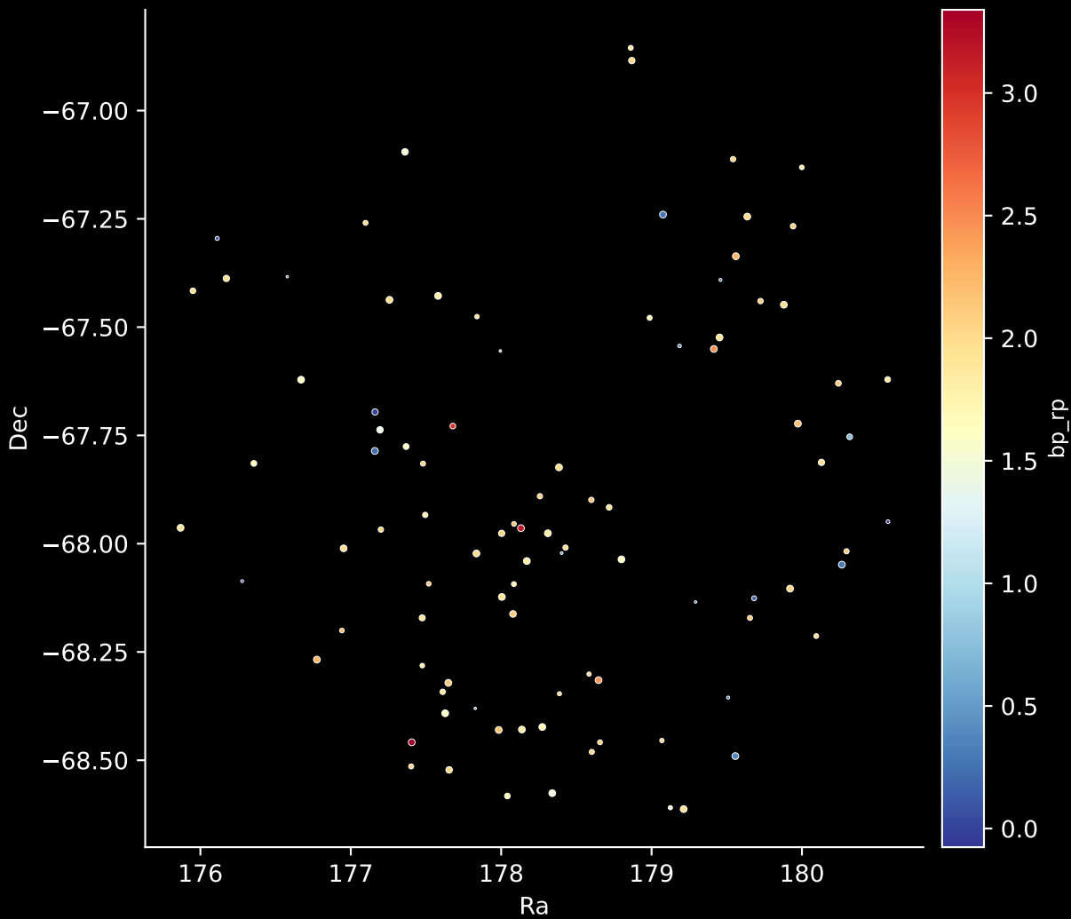
APOGEE DR17 Field: [LMC27] Stars: 94
