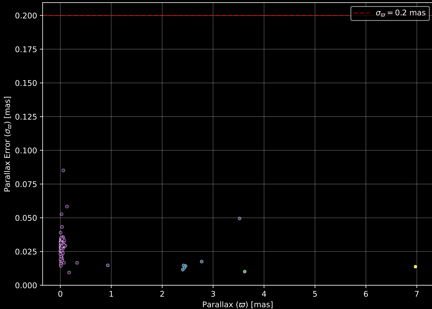
APOGEE DR17 Field: [LMC27] Parallax Quality (n= 94)
